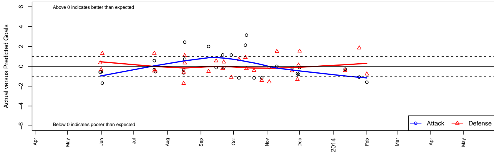
SSC Shadow A Navy B95 Dots are actual minus expected GF (blue circles) and GA (red triangles). Blue line is smoothed change in attack strength. Red is smoothed change in defense strength.
